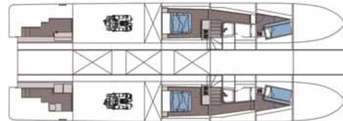
Lower Deck
